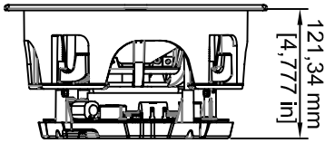
IC-62 without back box with round grille
