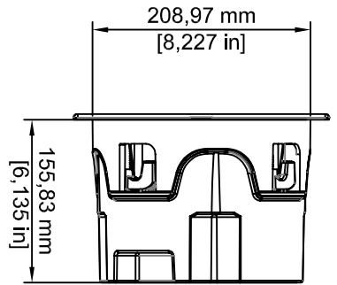
IC-62 with Back box with round grille
