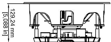
IC81 and IC82 without back box, with round grill
