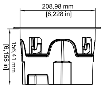
IC61 with back box
