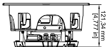
IC61 without back box
