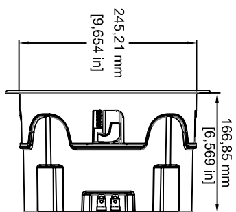
IC81 and IC82 with back box and round grill
